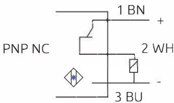
electric diagram
